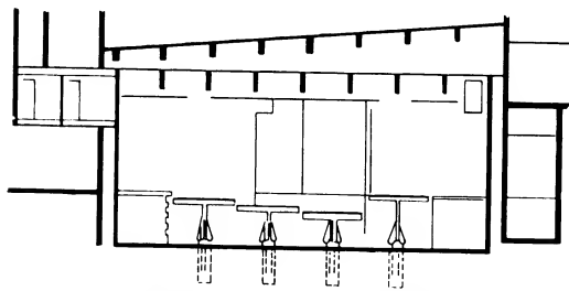
④ Podium in the theatre at Ulm (longitudinal section)
